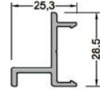
635-6101 (0,325 kg/mt) IP35P01 KAPAK BASKI PRF. 8553
