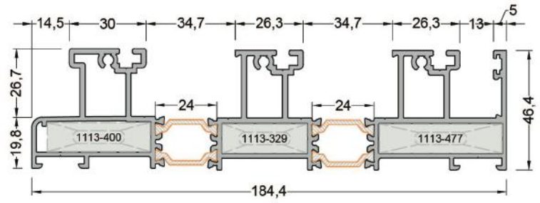
320-1302 ( 4,229 kg/mt ) SAT120 F05 3'LÜ KASA PROFİLİ
