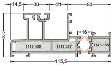
320-1102 ( 2,542 kg/mt ) SAT120 F10 MONORAIL KASA PROFİLİ
