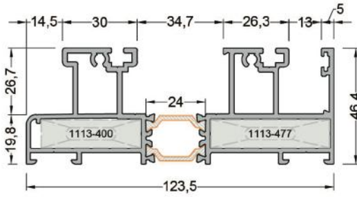
320-1202 ( 2,875 kg/mt ) SAT120 F07 2'LI KASA PROFİLİ
