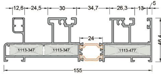
320-1203 ( 3,351 kg/mt ) SAT120 F11 SİNEKLİK RAYLI 2 Lİ KASA PROFİLİ
